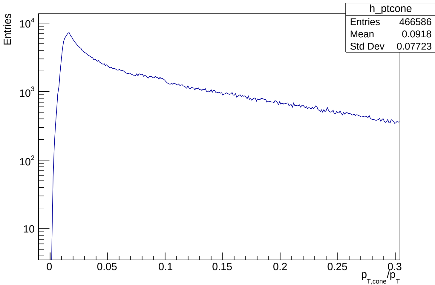
Distribution of Transverse Momentum Isolation of Leptons
